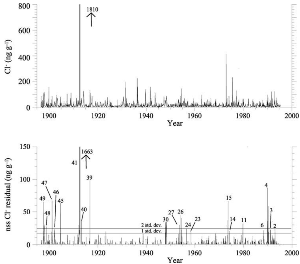
Figure 7. Volcanic \text{Cl}^- signals in the Eclipse ice core: (top) raw \text{Cl}^- time series; (bottom) nss \text{Cl}^- residuals ( \text{ng g}^{-1} ), 1 and 2 standard deviations above the mean as indicated. Numbering corresponds to event numbering in Table 3.
